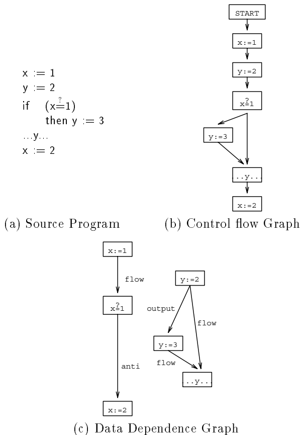
Figure 3: A Small Program and its Representations
