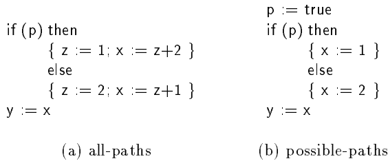
Figure 1: Examples of runtime constants
