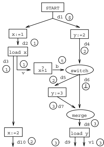
Figure 10: Result of Constant Propagation in Figure 5
