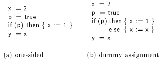
Figure 4: Transforming a one-sided conditional
