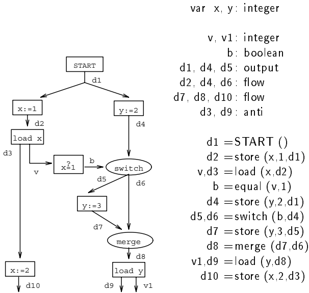
Figure 5: Dependence Flow Graph for a Small Program
