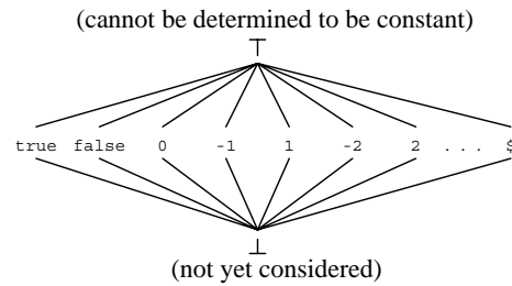
Figure 2: Lat — Lattice for constant propagation
