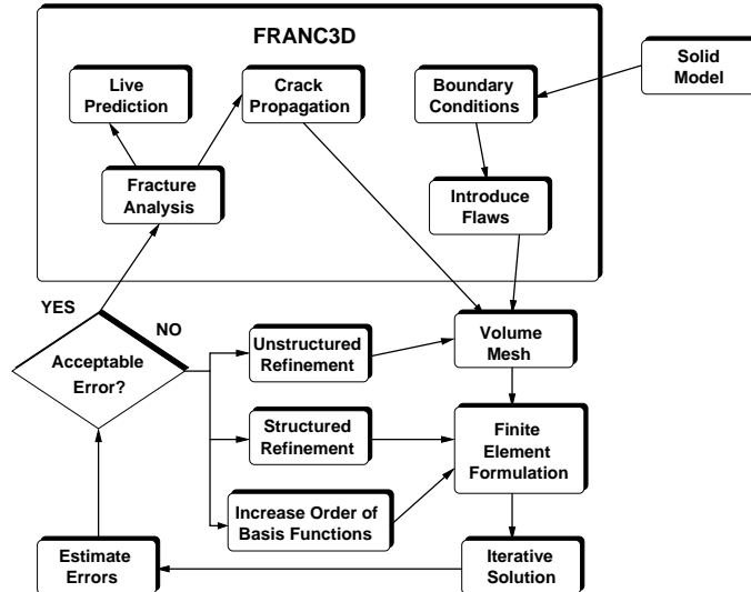
Figure 1: Simulation loop.
